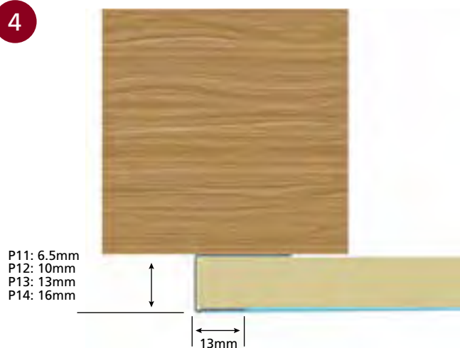
■ STOPPING BEAD DETAIL
