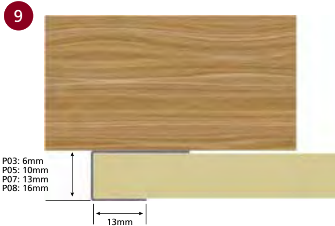
■ CASING BEAD DETAIL
