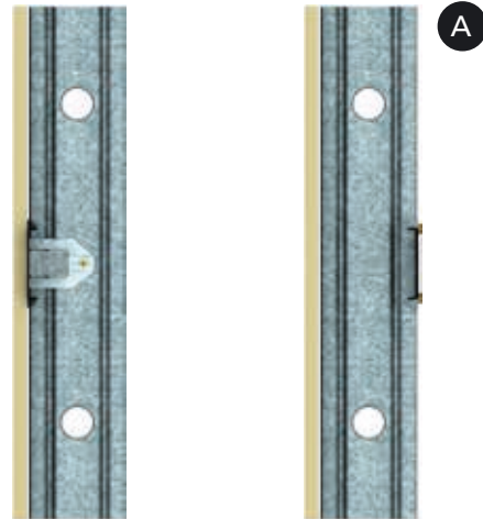
■ DETAIL SHOWING WALLS LINED ONE SIDE TO FULL HEIGHT
