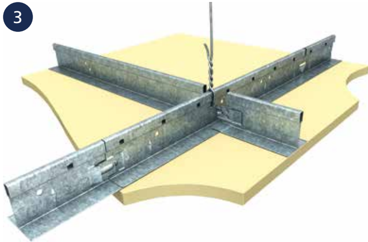
■ MAIN TEE & CROSS TEE INTERSECTION
