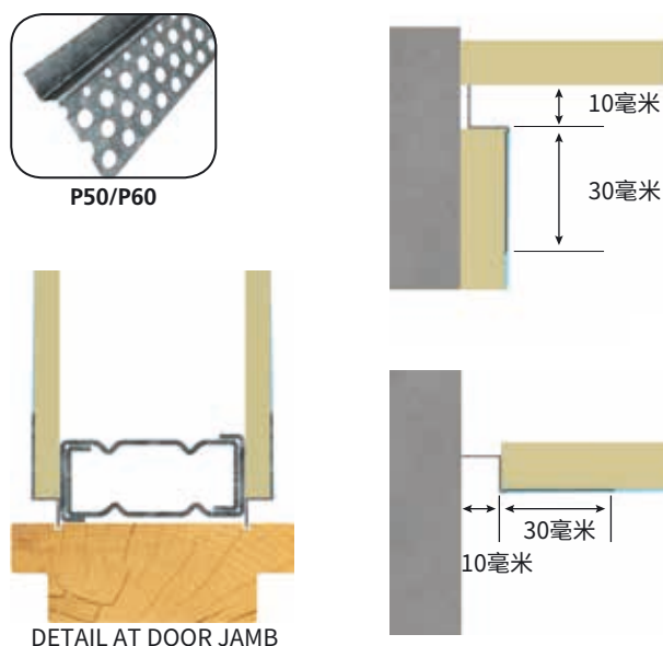
DETAIL AT DOOR JAMB
