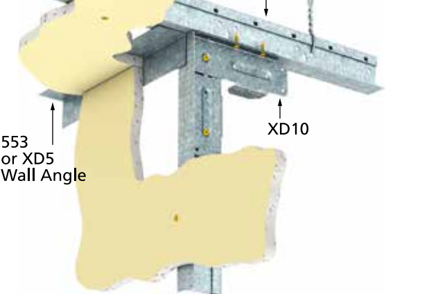
■ 90° INSIDE CORNER USING XD10
